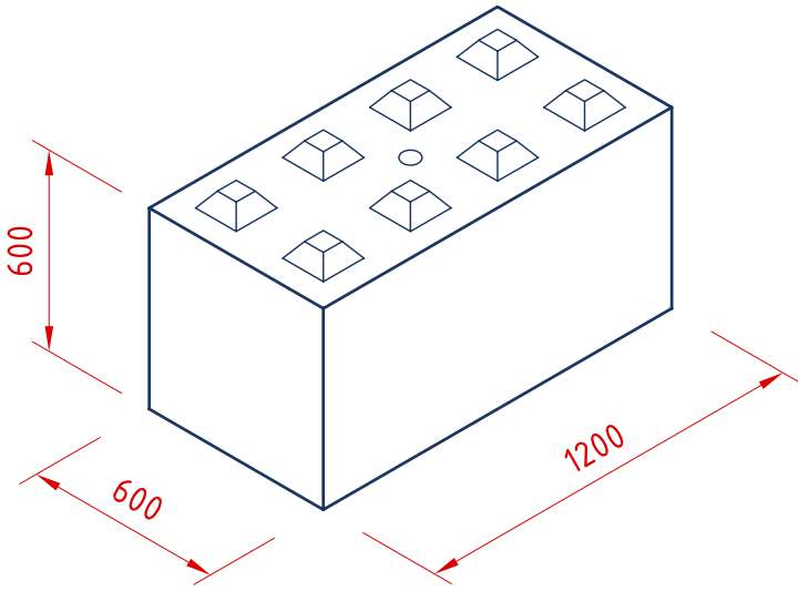
Block Type C ISOMETRIC VIEW
