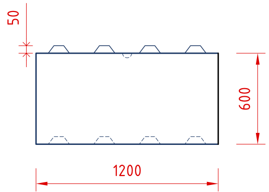
All Block Types END VIEW
